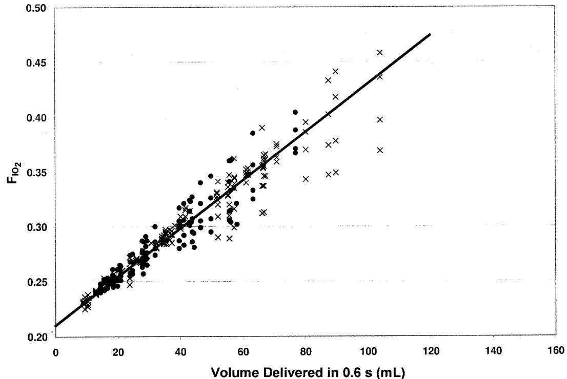
Fig. 5. Fraction of inspired oxygen ( F_{I_{O_2}} ) delivered with a volume-based setting system, during the initial 0.6 s. Dots represent measurements from demand-type systems. Xs represent measurements from pulse-type systems. When volume output during the first 0.6 s is plotted against F_{I_{O_2}} , the relationship is more direct ( r^2 = 0.92 ) than the volume-based system (see Fig. 4) or the setting-based system (see Fig. 3), even with both pulse-type and demand-type models combined in the analysis.
