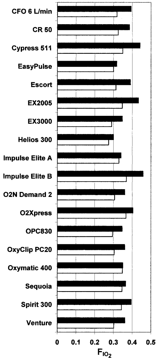
Fig. 2. Fraction of inspired oxygen (F IO 2 ) at the maximum output setting with continuous-flow oxygen and the tested demand oxygen delivery systems. The black bars represent F IO 2 measurements taken at 15 breaths/min. The white bars represent F IO 2 measurements taken at 30 breaths/min. F IO 2 differed markedly among the devices at their maximum settings. The higher respiratory frequency reduced F IO 2 with all the devices tested. The Oxymatic 401 and 411 operate the same at their maximum settings, so only one entry is shown. The same is true for the Sequoia 302 and 311.
