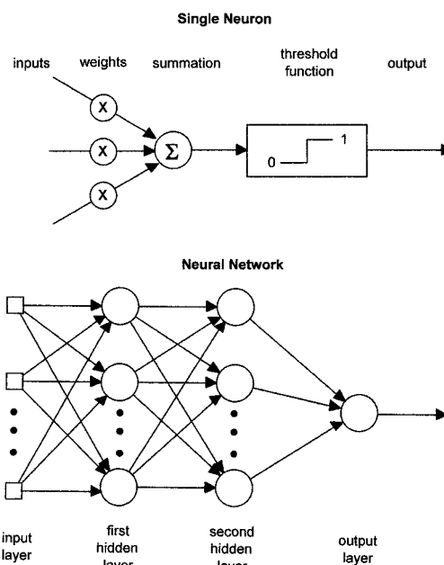
Fig. 10. Neural network structure. A single "neuron" accepts inputs of any value and weights them to indicate the strength of the synapse. The weighted signals are summed to produce an overall unit activation. If this activation exceeds a certain threshold the unit produces an output response. A network is made up of layers of individual "neurons."
